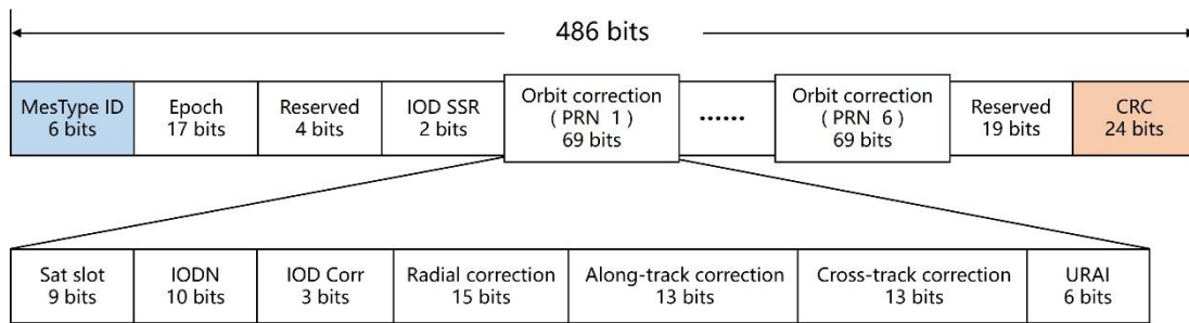
Fig B.2 Layout of PPP-B2b message type 2
