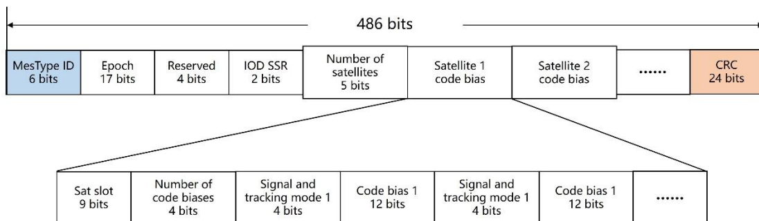
Fig B.3 Layout of PPP-B2b message type 3
