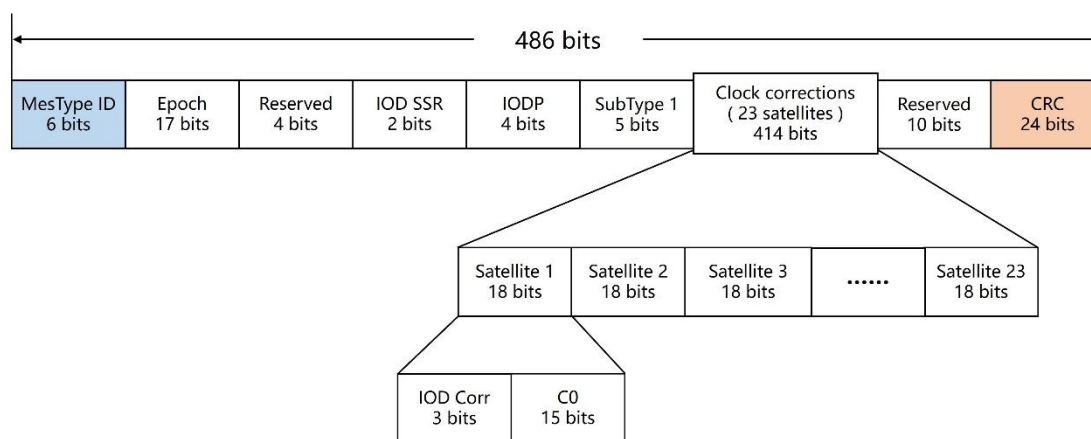
Fig B.4 Layout of PPP-B2b message type 4
